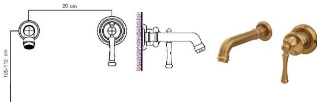
BASIN MIXER
